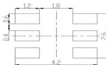
Soldering patterns
