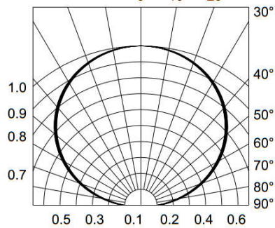
Fig.6-Radiation Diagram T_a=25^{\circ}\text{C}
